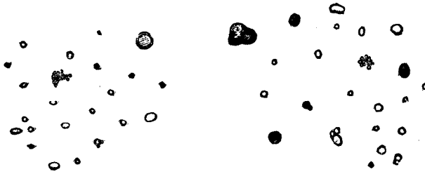
Fig. 181. Atmospheric Dust Greatly Magnified.
