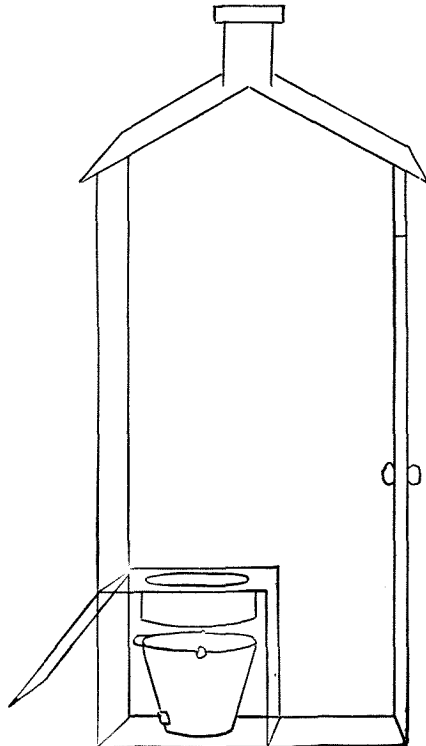
Fig. 183. Dry-Earth Pail in Position.
